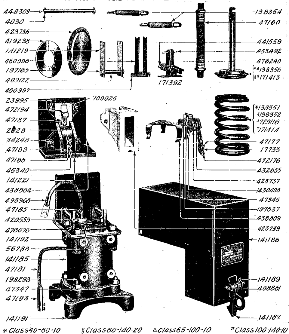
TYPE ML FORM A1 AIR COMPRESSOR GOVERNOR
