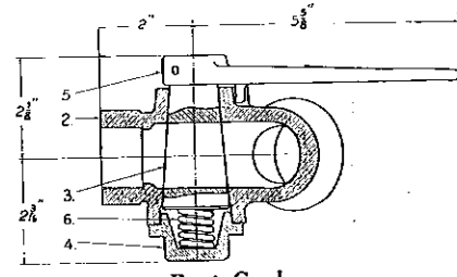
Bent Cock with Side Handle.
