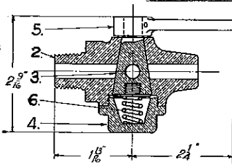
½" Drain Cock.
